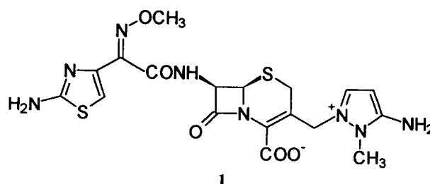
Figure 1. Structure of 7β-[(Z)-2-(2-aminothiazol-4-yl)-2-methoxyiminoacetamido]-3-(3-amino-2-methylpyrazolio)methyl-3-cephem-4-carboxylate ( 1 ).
